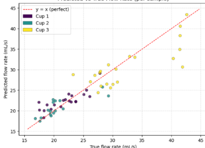
Predicted vs True Flow Rate (per sample)
