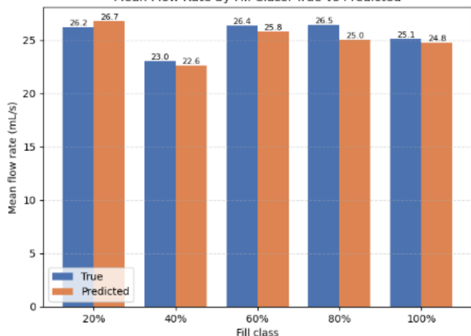
Mean Flow Rate by Fill Class: True vs Predicted
